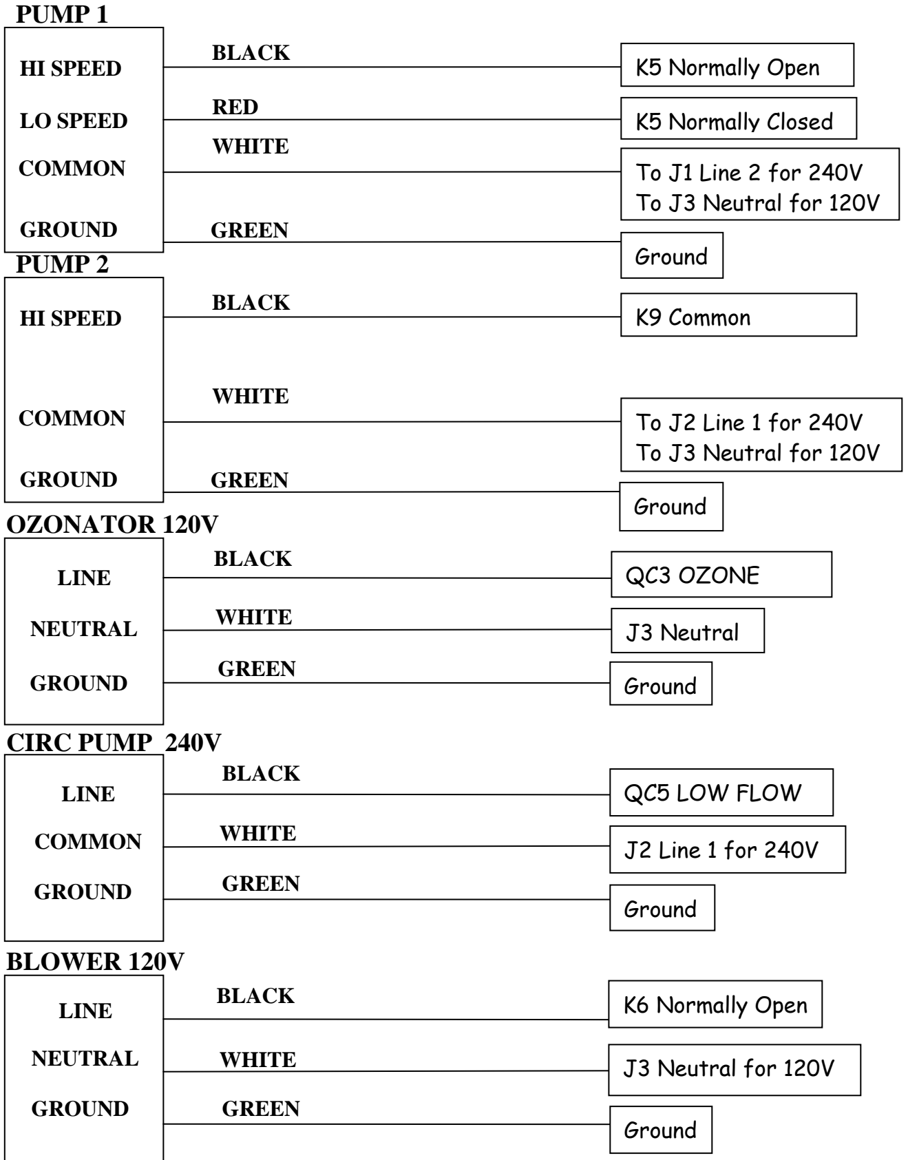
Receptacle Connection Diagram
