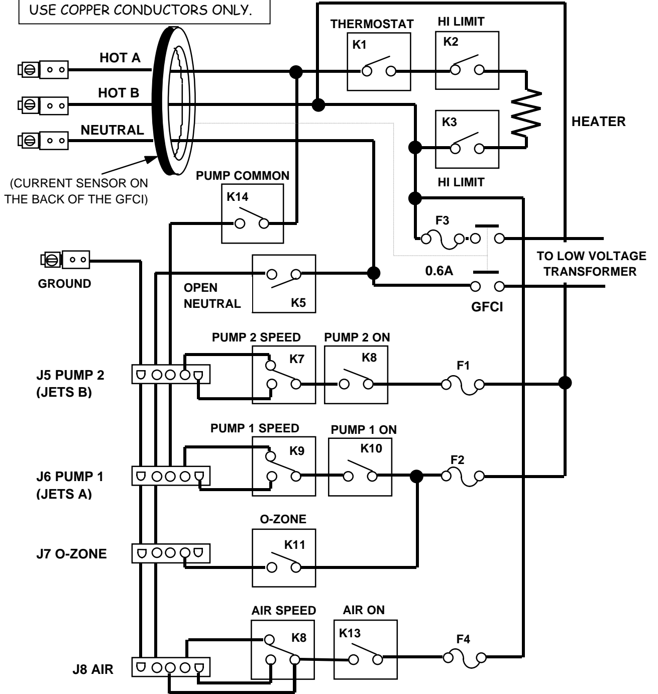
P2P-G39 AC WIRING
