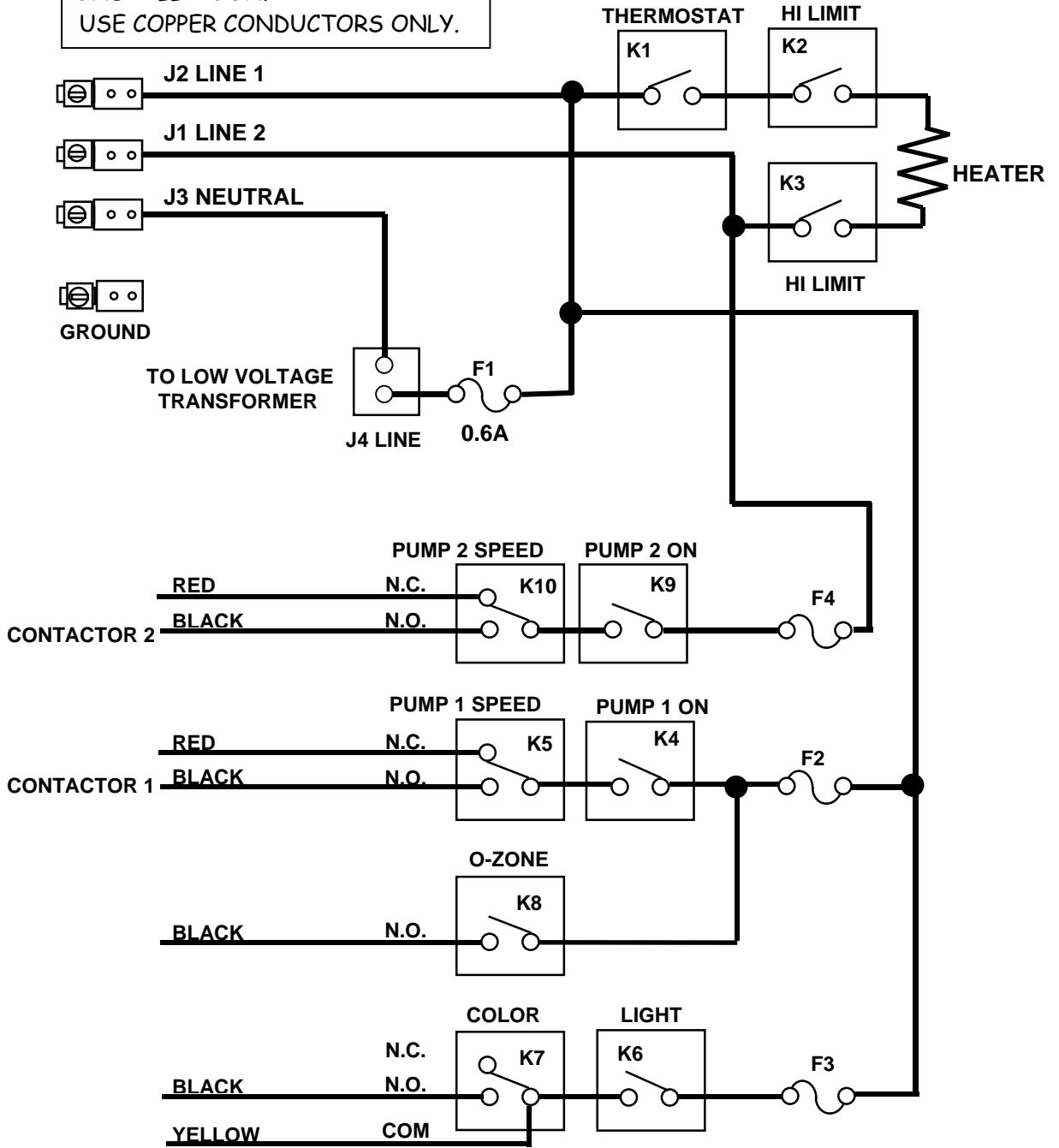
P2P-N46 AC WIRING
