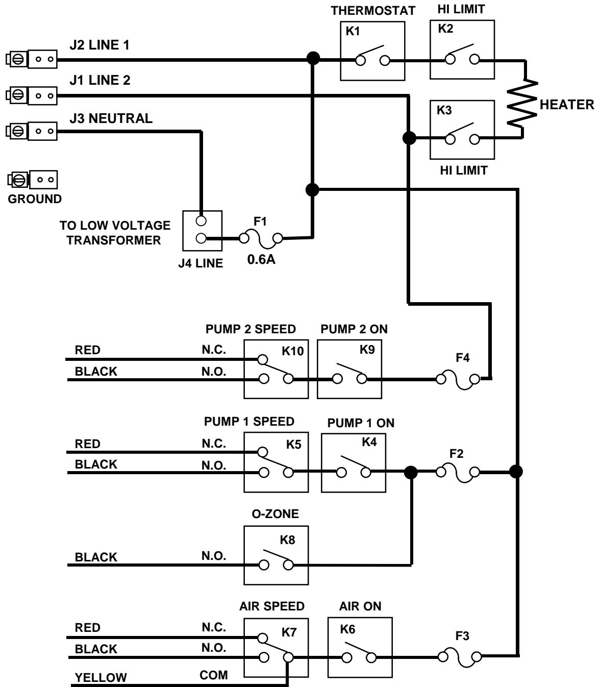
P2P-N46 AC WIRING
